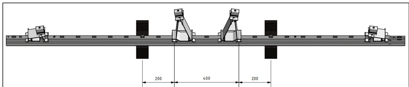
Vista lateral 2400mm pitch
