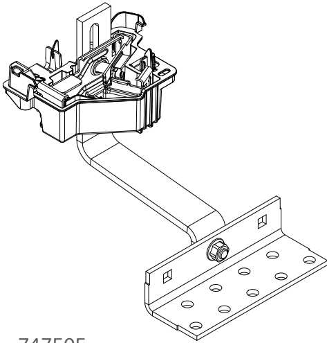
747505 ValkAce+ - Strongline dakhaak
